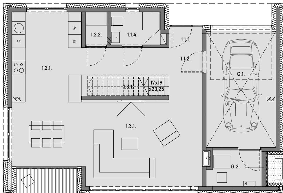
parter
